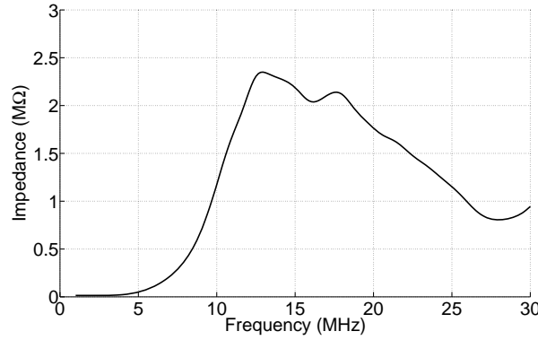
Figure 4.29: Impedance of RF compensated Langmuir probe.
