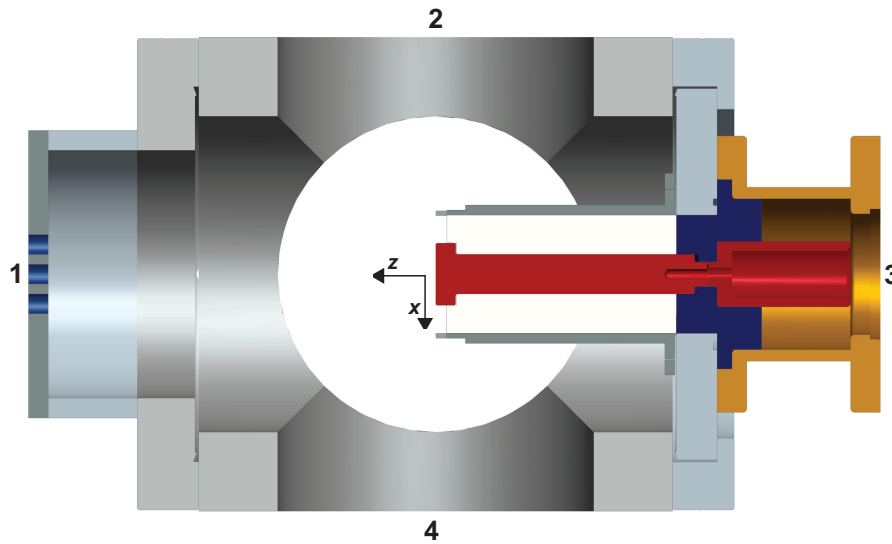
Figure 4.1: Experimental setup for the parallel field configuration.
