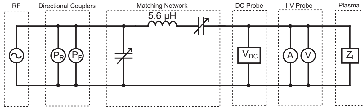
Figure 4.5: Circuit diagram of the RF system.
