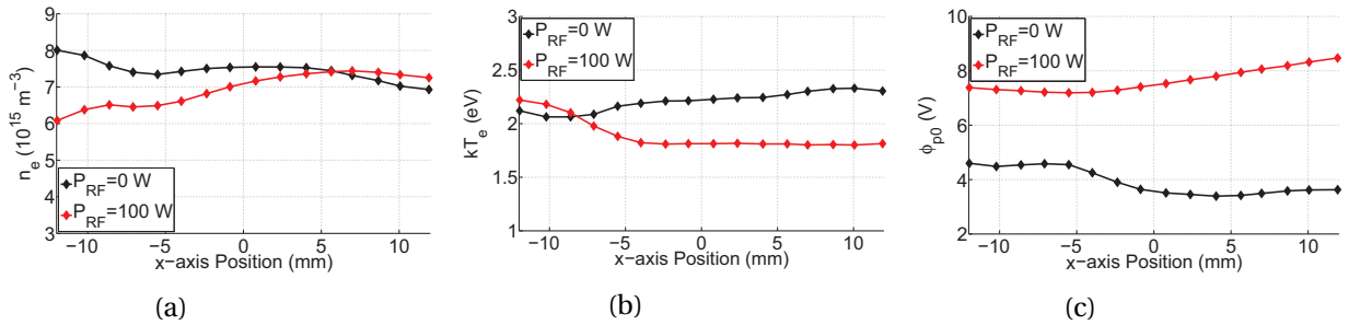
Figure 5.16: Spatial distribution of (a) n_e , (b) kT_e , and (c) \phi_{p0} for hydrogen in the perpendicular field configuration.
