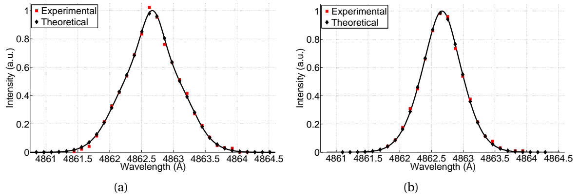
Figure D.17: Fit to the H_{\beta} (a) \pi and (b) \sigma profiles for shot 20 at a position of z = 4.1 mm.
