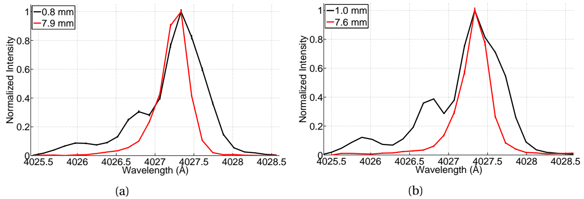
Figure 5.40: 5^3D \rightarrow 2^3P He I \pi profiles at z = 0.8 mm and 7.9 mm and (b) z = 1.0 and 7.6 mm in the parallel and perpendicular field configurations respectively.
