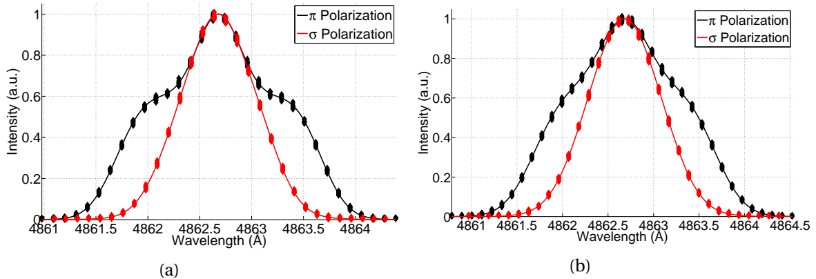
Figure 5.50: H_\beta \pi and \sigma profiles for E_0 = E_1 = 3.3 kV/cm and (a) kT_{R1} = 1.0 and (b) 2.0 eV with simulated noise.
