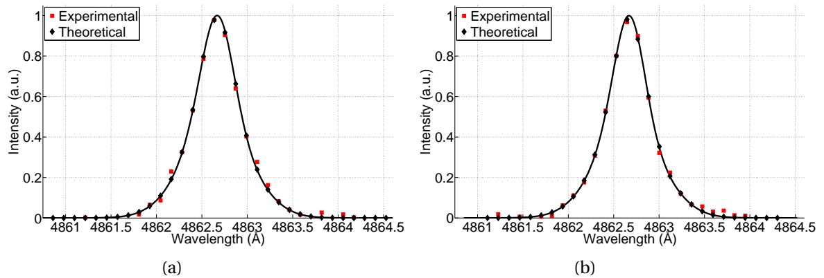
Figure D.18: Fit to the H_{\beta} (a) \pi and (b) \sigma profiles for shot 20 at a position of z = 7.6 mm.
