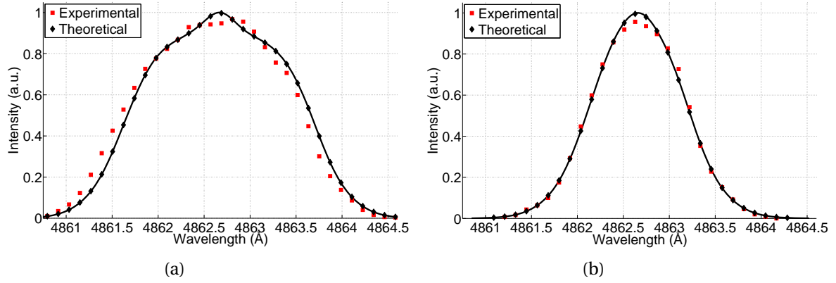
Figure D.16: Fit to the H_{\beta} (a) \pi and (b) \sigma profiles for shot 20 at a position of z = 1.0 mm.
