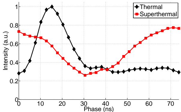
Figure 5.47: Thermal and superthermal emission as a function of phase in the parallel field configuration.
