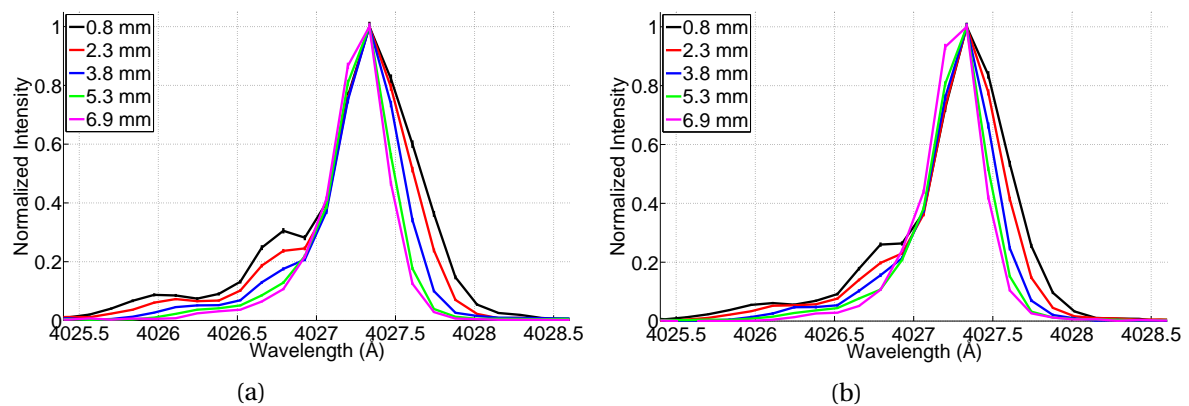
Figure 5.35: 5^3D \rightarrow 2^3P He I spectral line profile as a function of position in the RF sheath for the (a) \pi and (b) \sigma components in the parallel field configuration.
