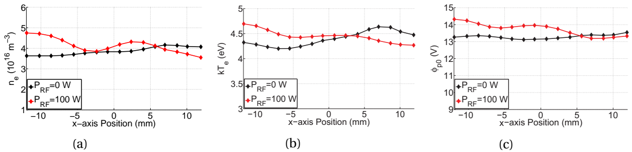
Figure 5.17: Spatial distribution of (a) n_e , (b) kT_e , and (c) \phi_{p0} for helium in the perpendicular field configuration.
