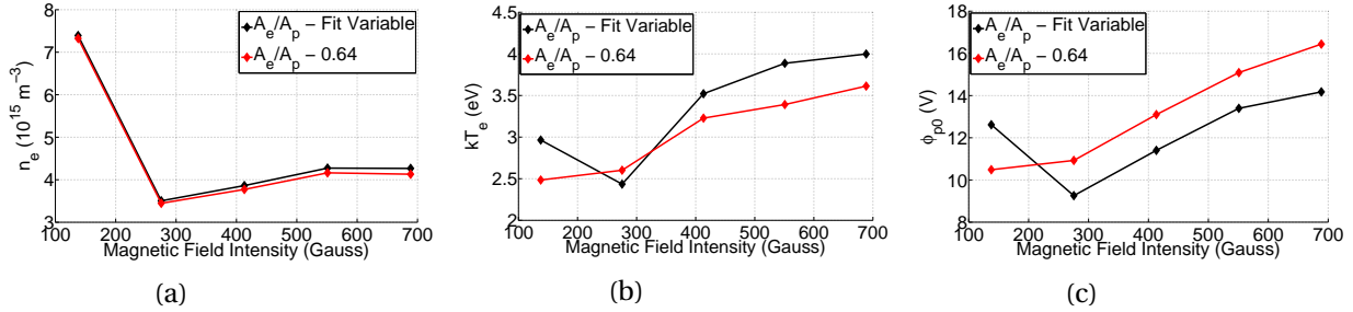
Figure 5.12: (a) n_e , (b) kT_e , and (c) \phi_{p0} associated with the variable and constant A_e fit scenarios.
