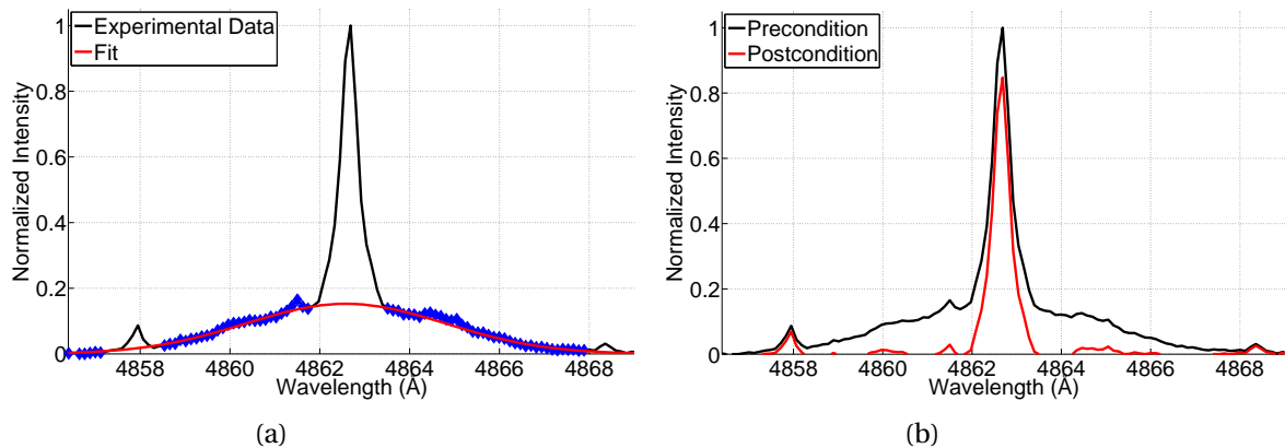
Figure 5.23: H β π spectral line profile at a position of z = 7.9 mm in the parallel field configuration showing the (a) superthermal emission fit and (b) removal.
